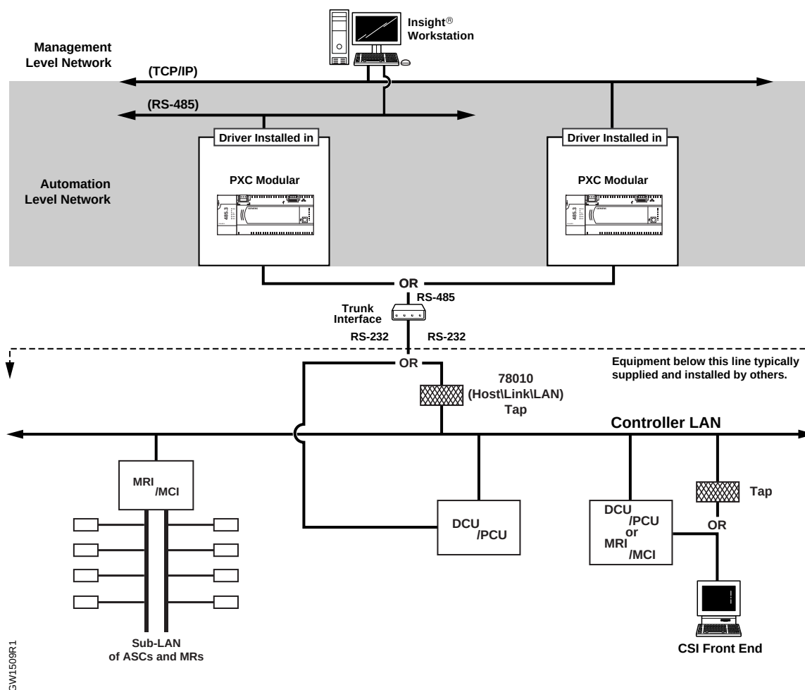
Figure 1. Typical System Architecture — Recommended (Firmware Revision 2.x).
