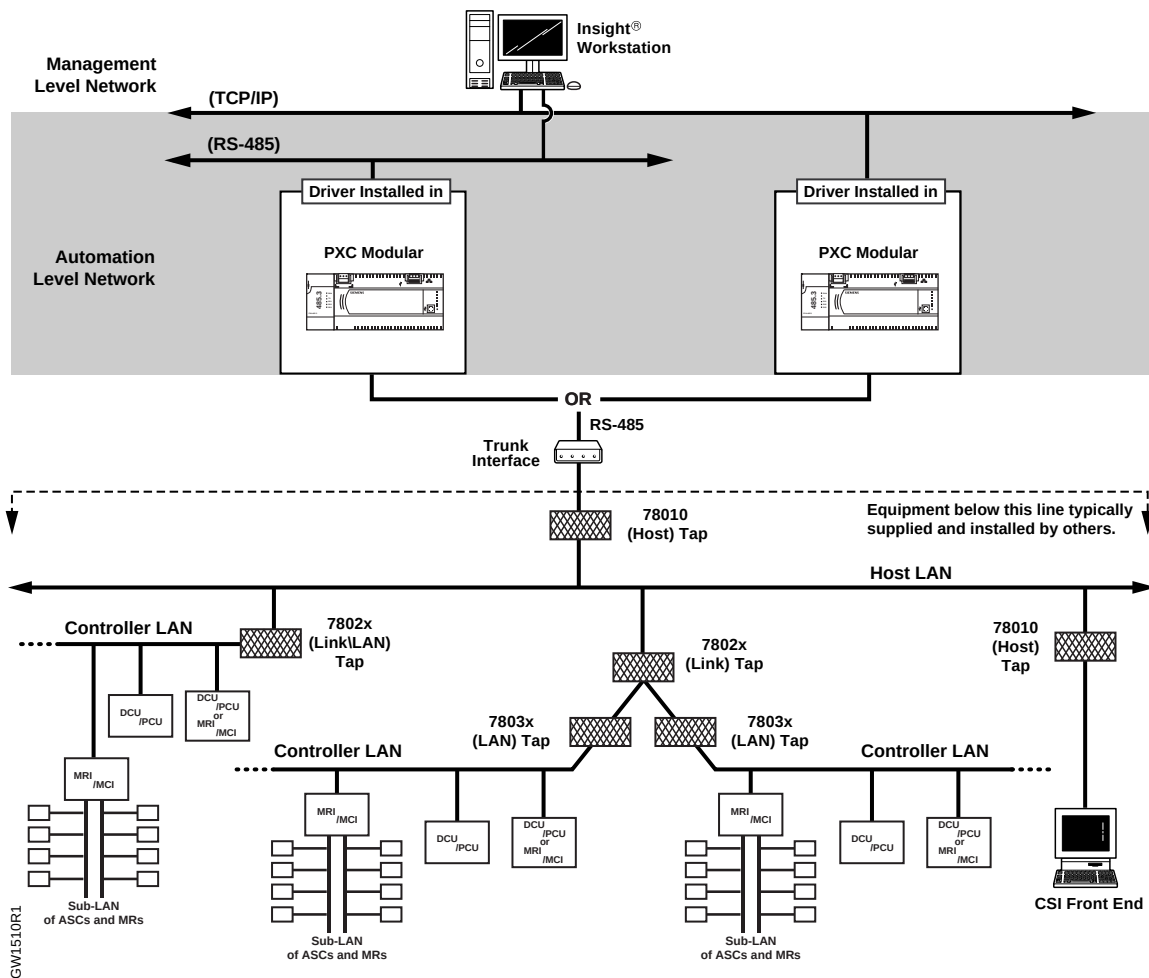
Figure 2. Alternate System Architecture (Firmware Revision 2.x).
