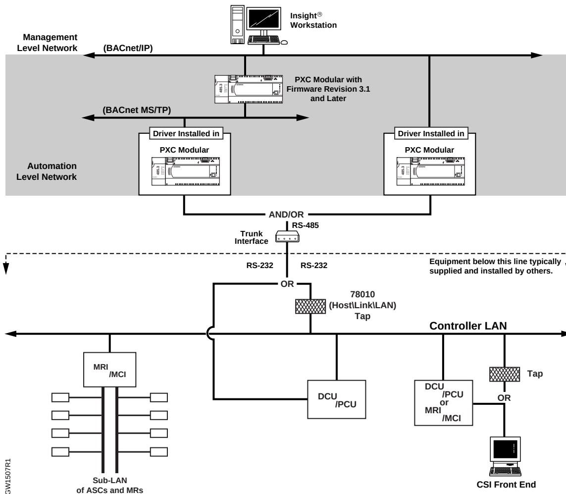
Figure 3. Typical System Architecture — Recommended (Firmware Revision 3.x).
