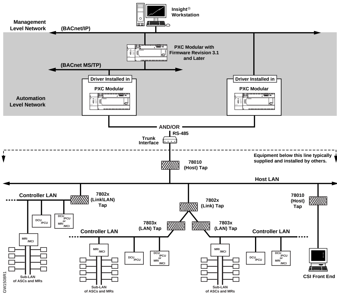
Figure 4. Alternate System Architecture (Firmware Revision 3.x).
